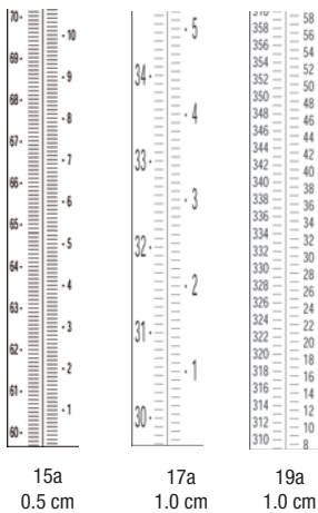
Available Invar rod graduations
